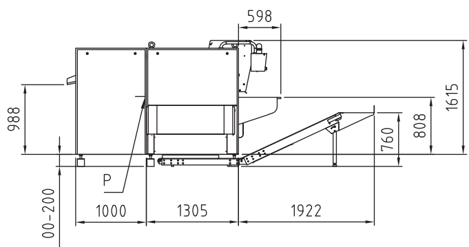
(Amfold-B Amstack-D/Left)
